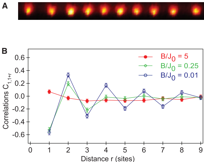
Fig. 3. Quantum phase transition from a paramagnet to an antiferromagnet (Eq. 1), with J_{ij} \approx |i - j|^{-1.05} in a system of 10 spins. The exponent ( \alpha = 1.05 ) is estimated from the average couplings between spins in this inhomogeneous system. (A) Image of 10 trapped ions, with a distance of 22 \mu\text{m} between the first and last ion. (B) Measured two-point correlation function between a chosen spin (on the edge) and the other spins separated by r lattice sites, C_{1,1+r} = \langle \sigma_x^{(1)} \sigma_x^{(1+r)} \rangle - \langle \sigma_x^{(1)} \rangle \langle \sigma_x^{(1+r)} \rangle , averaged over 4000 experiments for each value of the parameter B/J_0 . For B/J_0 = 5 , the spins are initially polarized along the transverse y field with little correlation along the Ising x direction. As the field is reduced, the spins cross over to pre-
