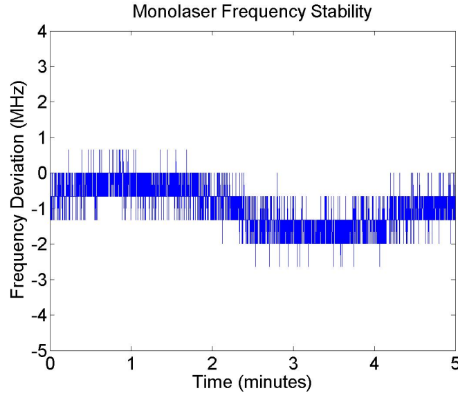
Figure 5-8: Monolaser frequency stability over a 5 minute period.
