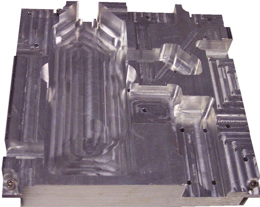
Figure 5-3: Photograph of the monolaser baseplate.
