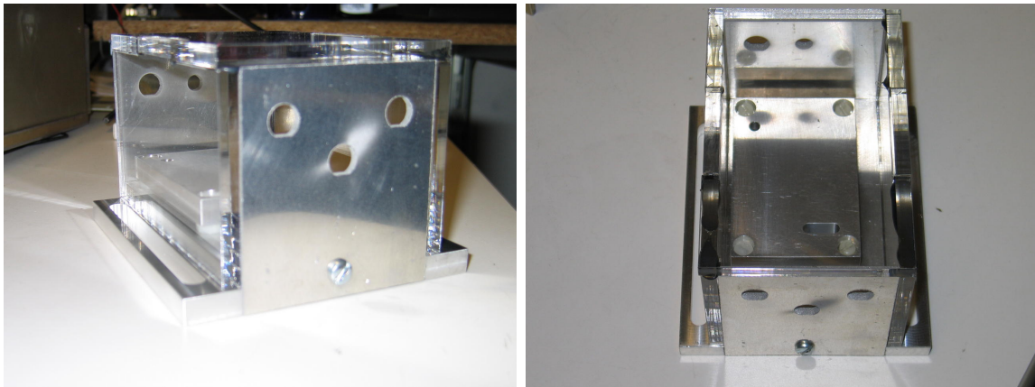
Figure 4-9: Photographs of the ECDL baseplate and housing. Laser optics are mounted on a small steel plate secured with teflon screws. A thermistor/TEC pair (not shown) are mounted on the baseplate to provide active temperature stabilization. The holes are sized to accept BNC bulkheads for internal electrical connections.
