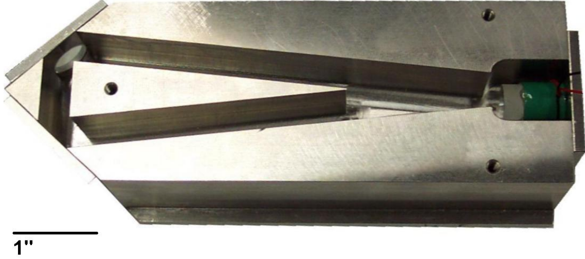
Figure 5-2: Photograph of the filter cavity.
