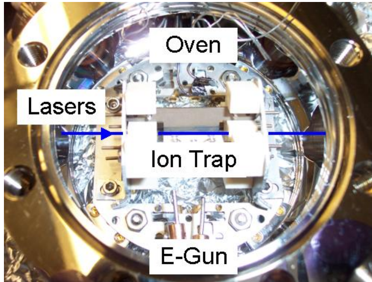
Figure 2-6: Picture of the trap chamber showing the strontium oven and electron gun. Collisions between the electrons and neutral strontium causes ionization at the trapping site.
