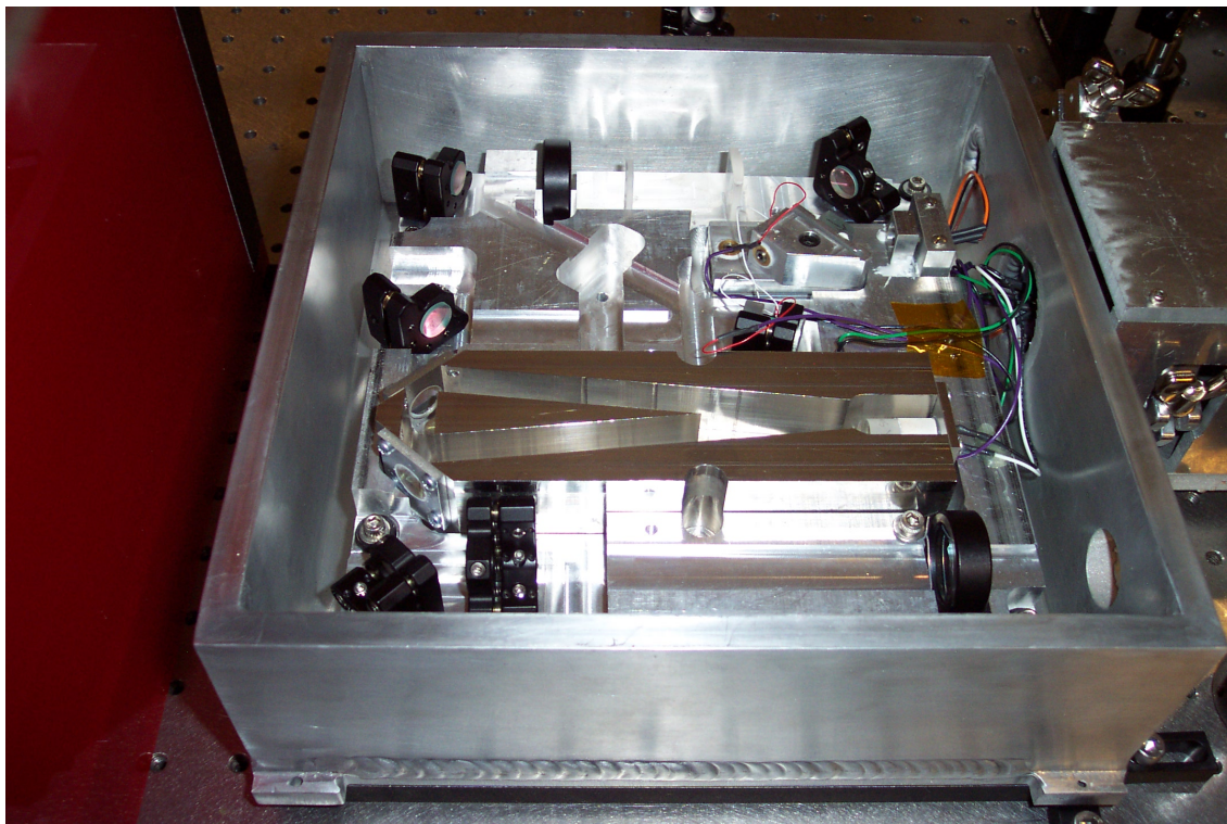
Figure 5-4: Photograph of the completed monolaser.
