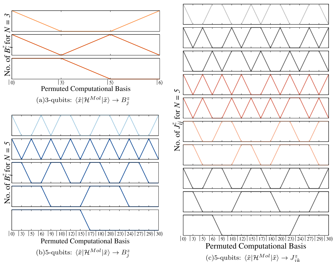
Figure 12. Transformation from \langle \tilde{x} | \mathcal{H}^{Mol} | \tilde{x} \rangle to the B^z -values for three qubits (a) and B^z (b) and J^z -values (c) for five qubits. This inverse matrix picks out the appropriate columns from the 2^{N-1} -dimensional Hadamard transformation matrix. See eqs 11 and B5. The B^z transformations (a, b) arise from two basic vectors (top and bottom). The vector in the bottom panel is scaled in frequency to create the other vectors. This aspect is shown using two different color shades. Similarly, J^z transformations (c) arise from five basic transformations arranged with different color shades in panels 1-3, 4-5, 6-7, 8-9, and 10.
